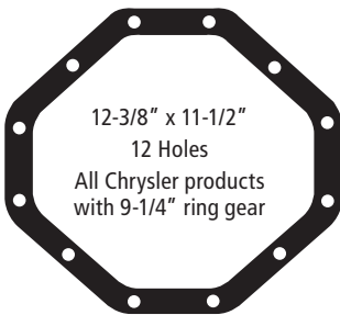
CHRYSLER 9-1/4"
