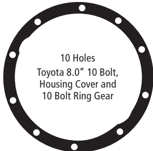
TOYOTA 8
