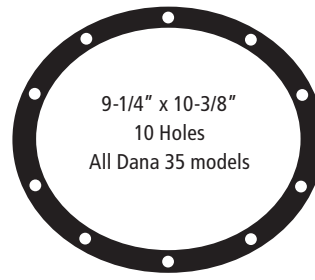
DANA 35
