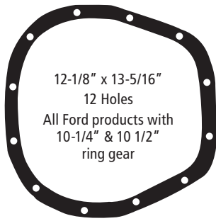
FORD 10-1/4", 10-1/2"
