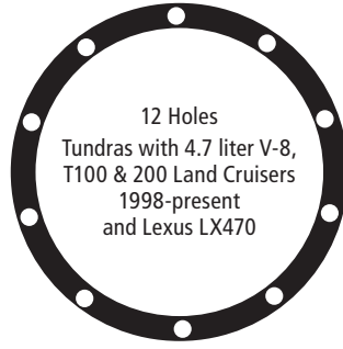
TOYOTA 9-1/2
