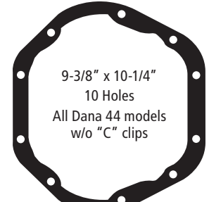
DANA 44
